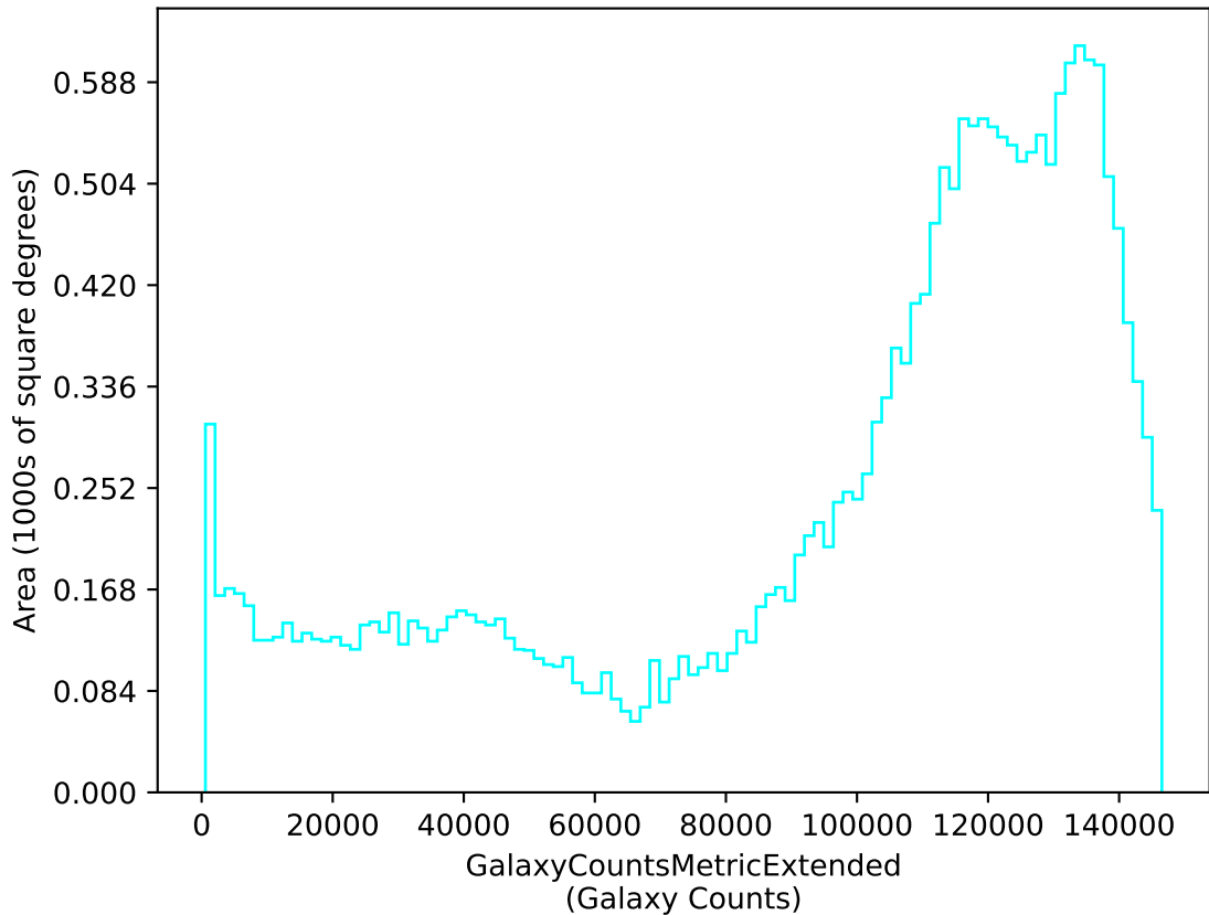
ddf_acor_sf15_lsf20_lsr20_v3.4_10yrs u: GalaxyCountsMetricExtended
