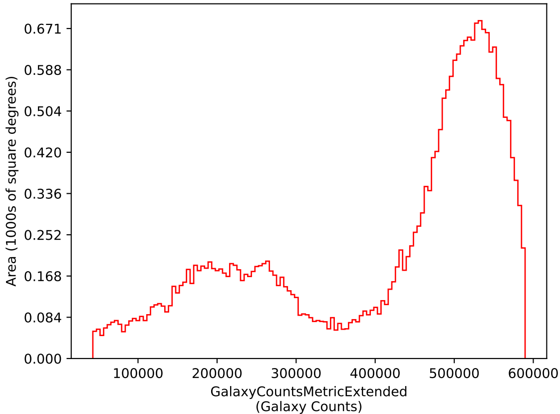
ddf_acor_sf15_lsf20_lsr20_v3.4_10yrs i: GalaxyCountsMetricExtended
