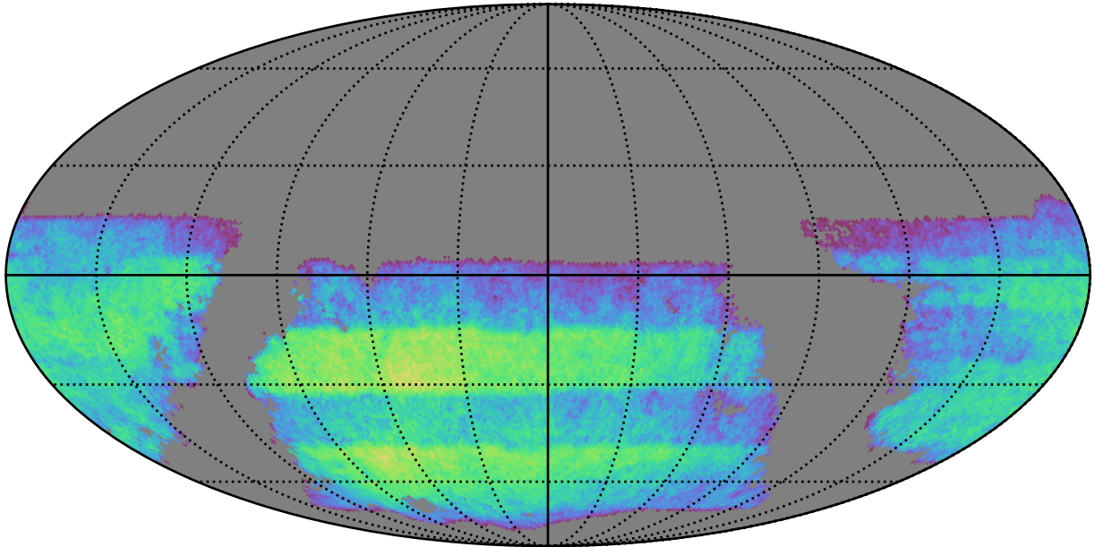
ddf_acor_sf15_lsf20_lsr20_v3.4_10yrs i band non-DD year 3: ExgalM5WithCuts
