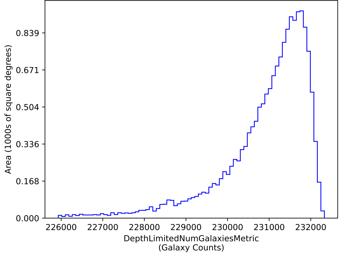
ddf_acor_sf15_lsf20_lsr20_v3.4_10yrs i band galaxies non-DD: DepthLimitedNumGalaxiesMetric
