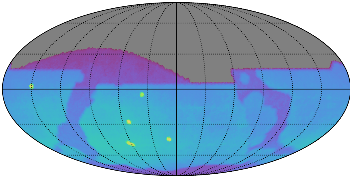
ddf_acor_sf15_lsf20_lsr20_v3.4_10yrs : Brown Dwarf, L7
