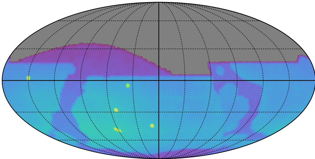
ddf_acor_sf15_lsf20_lsr20_v3.4_10yrs : Brown Dwarf, L4
