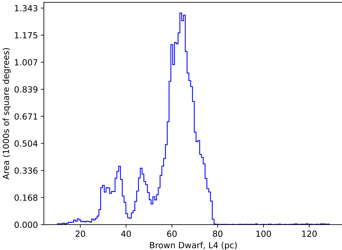
ddf_acor_sf15_lsf20_lsr20_v3.4_10yrs : Brown Dwarf, L4
