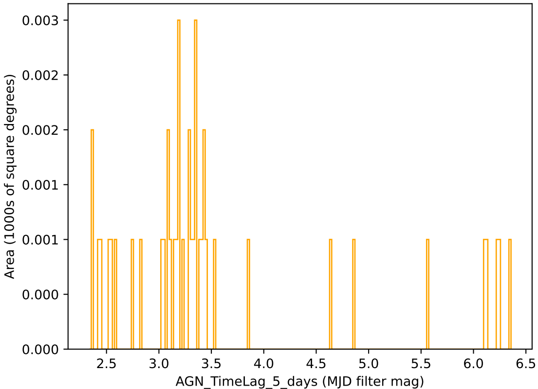
ddf_acor_sf15_lsf20_lsr20_v3.4_10yrs r band: AGN_TimeLag_5_days
