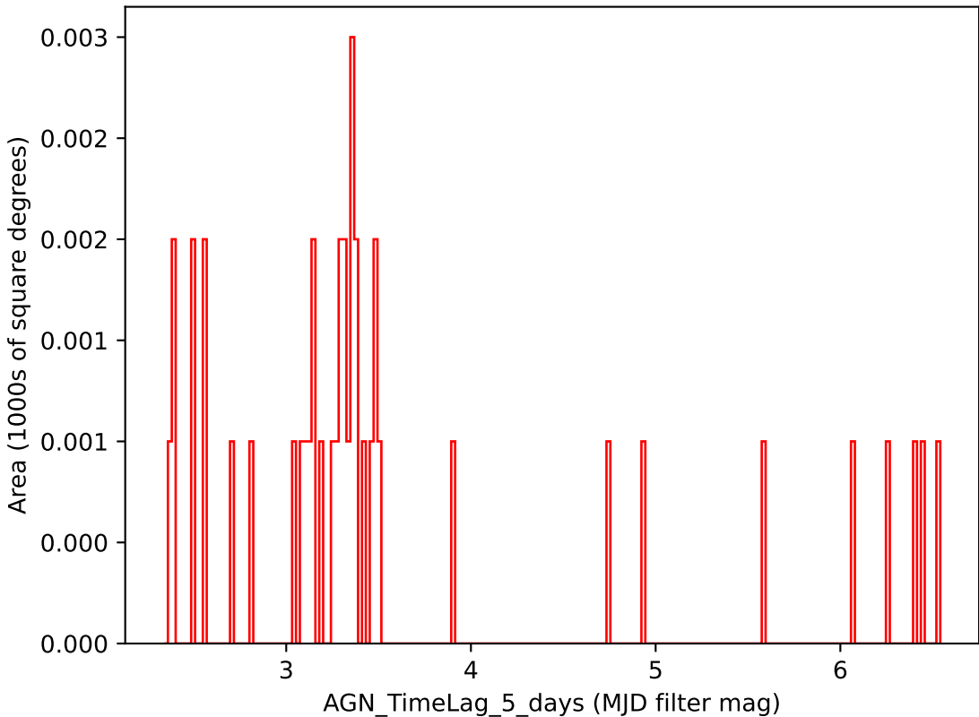
ddf_acor_sf15_lsf20_lsr20_v3.4_10yrs i band: AGN_TimeLag_5_days
