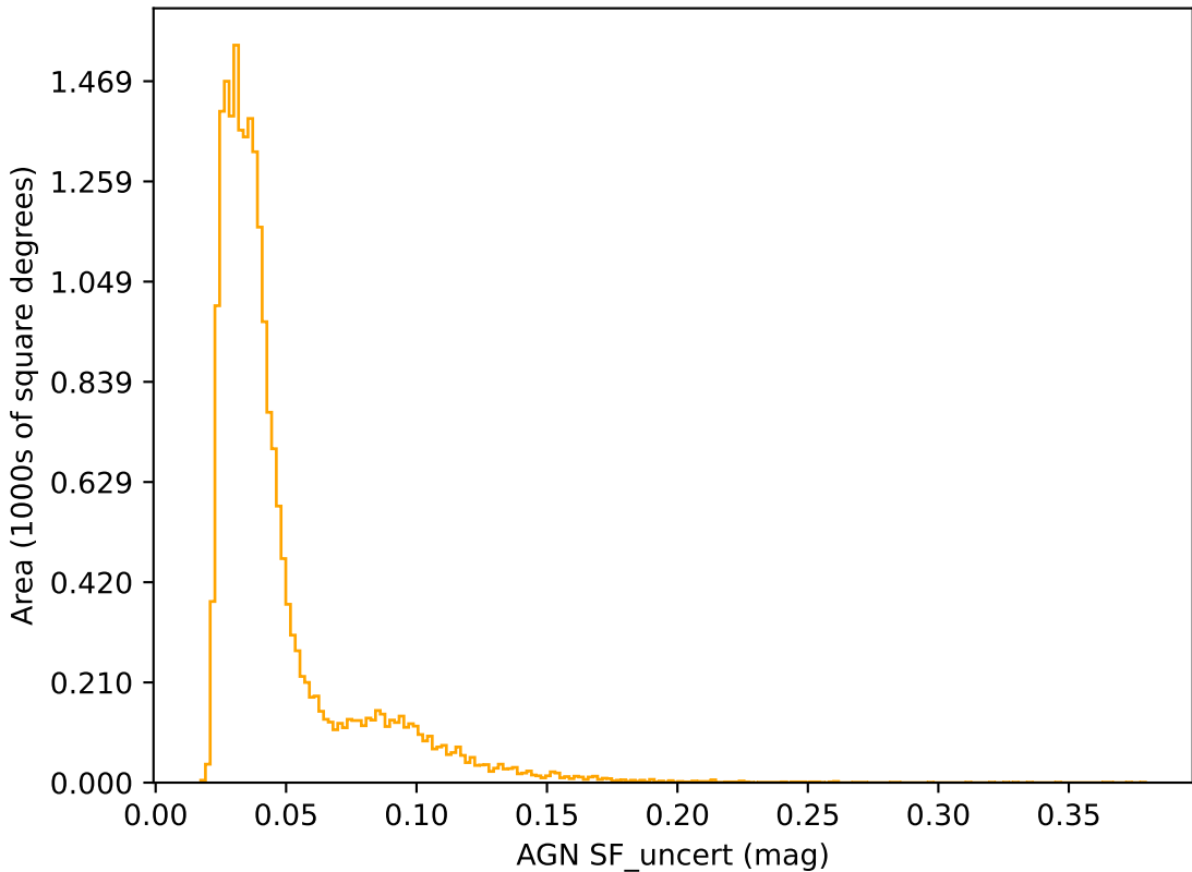
ddf_acor_sf15_lsf20_lsr20_v3.4_10yrs r band: AGN SF_uncert
