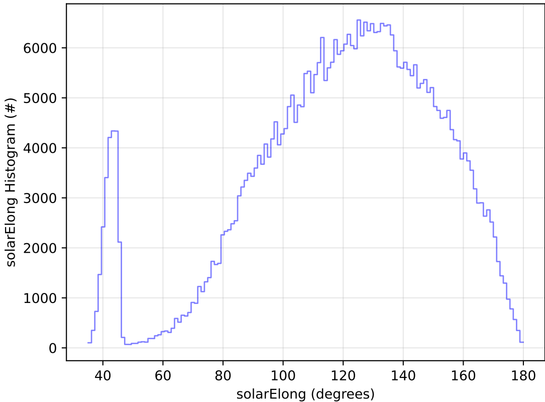
ddf_acor_sf15_lsf20_lsr20_v3.4_10yrs WFD z band: solarElong Histogram
