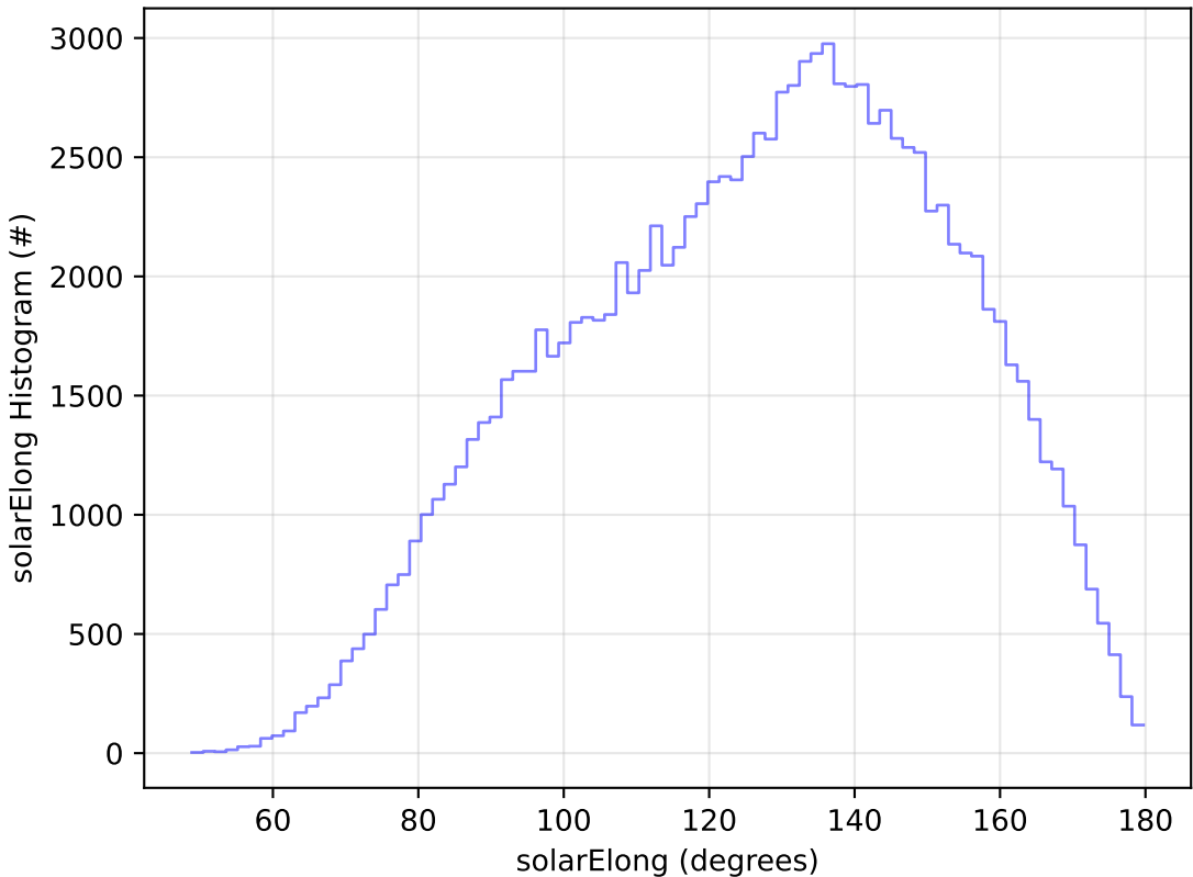
ddf_acor_sf15_lsf20_lsr20_v3.4_10yrs WFD u band: solarElong Histogram
