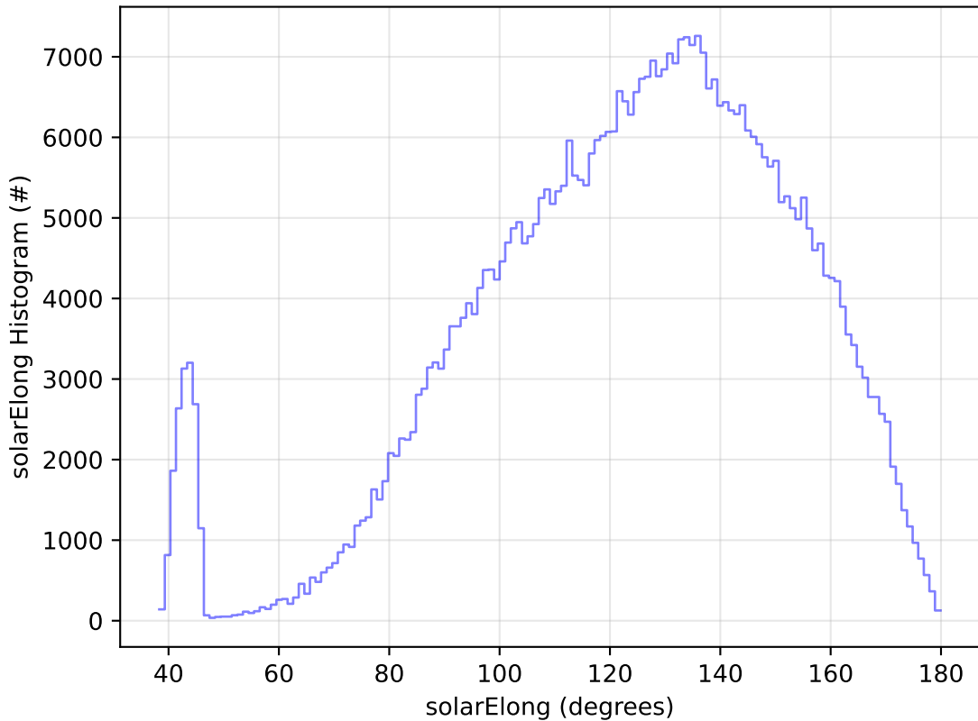
ddf_acor_sf15_lsf20_lsr20_v3.4_10yrs WFD r band: solarElong Histogram
