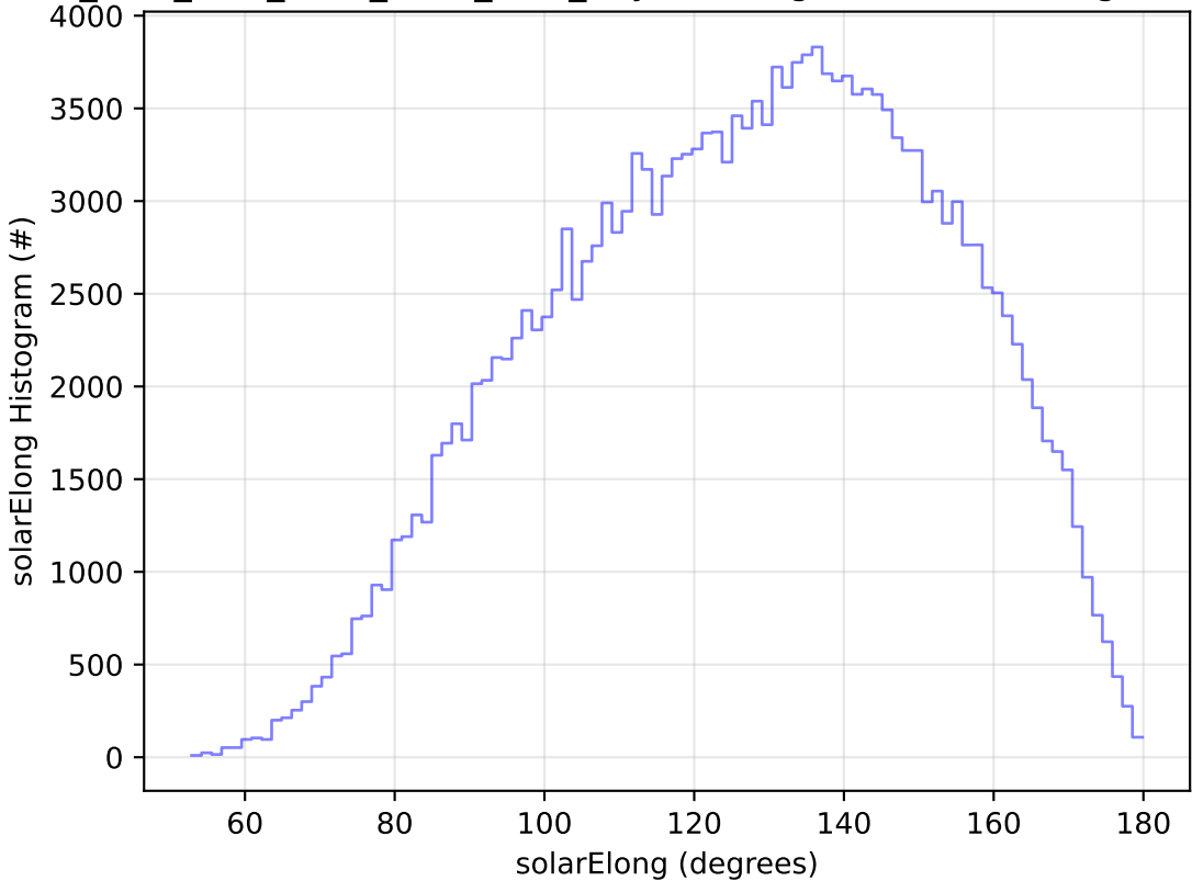
ddf_acor_sf15_lsf20_lsr20_v3.4_10yrs WFD g band: solarElong Histogram
