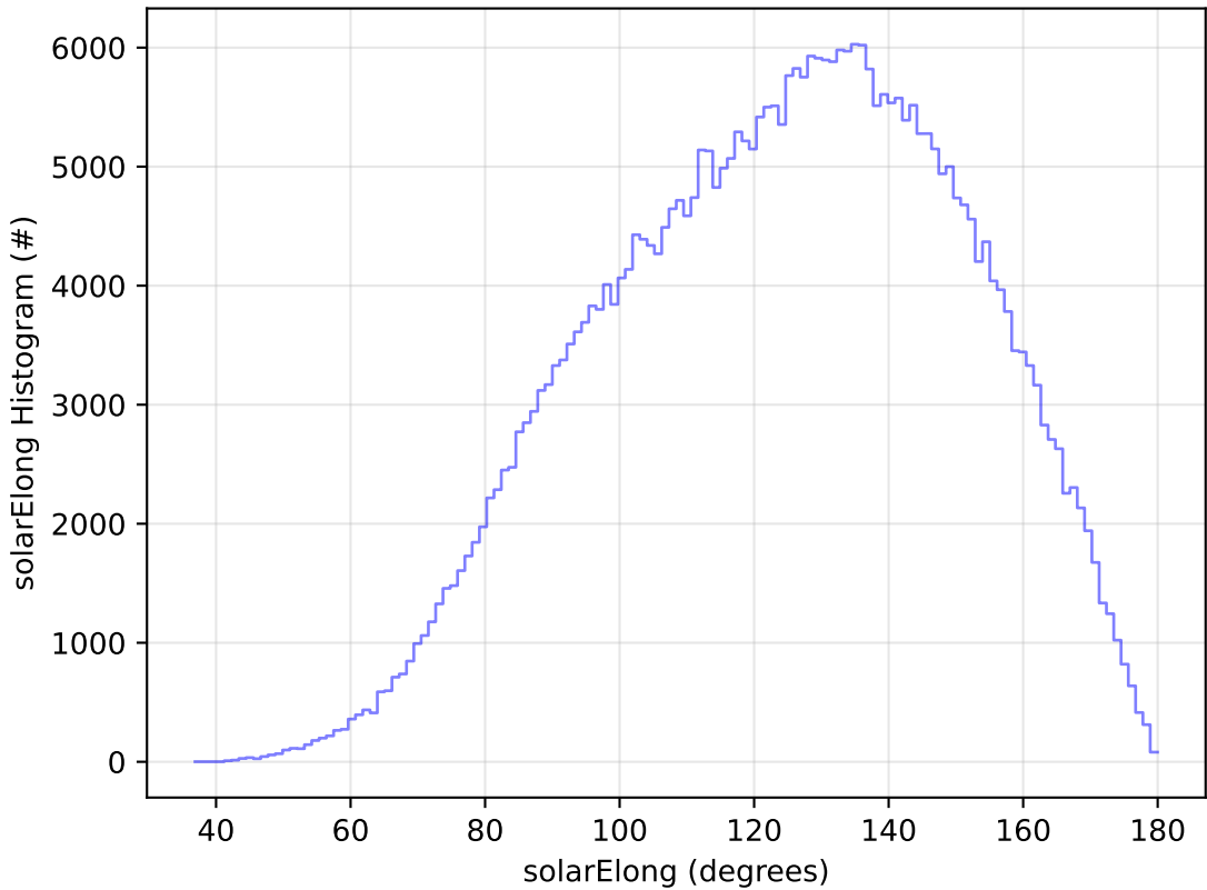
ddf_acor_sf15_lsf20_lsr20_v3.4_10yrs All sky y band: solarElong Histogram
