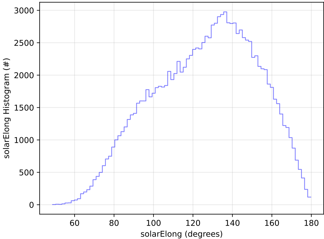
ddf_acor_sf15_lsf20_lsr20_v3.4_10yrs All sky u band: solarElong Histogram
