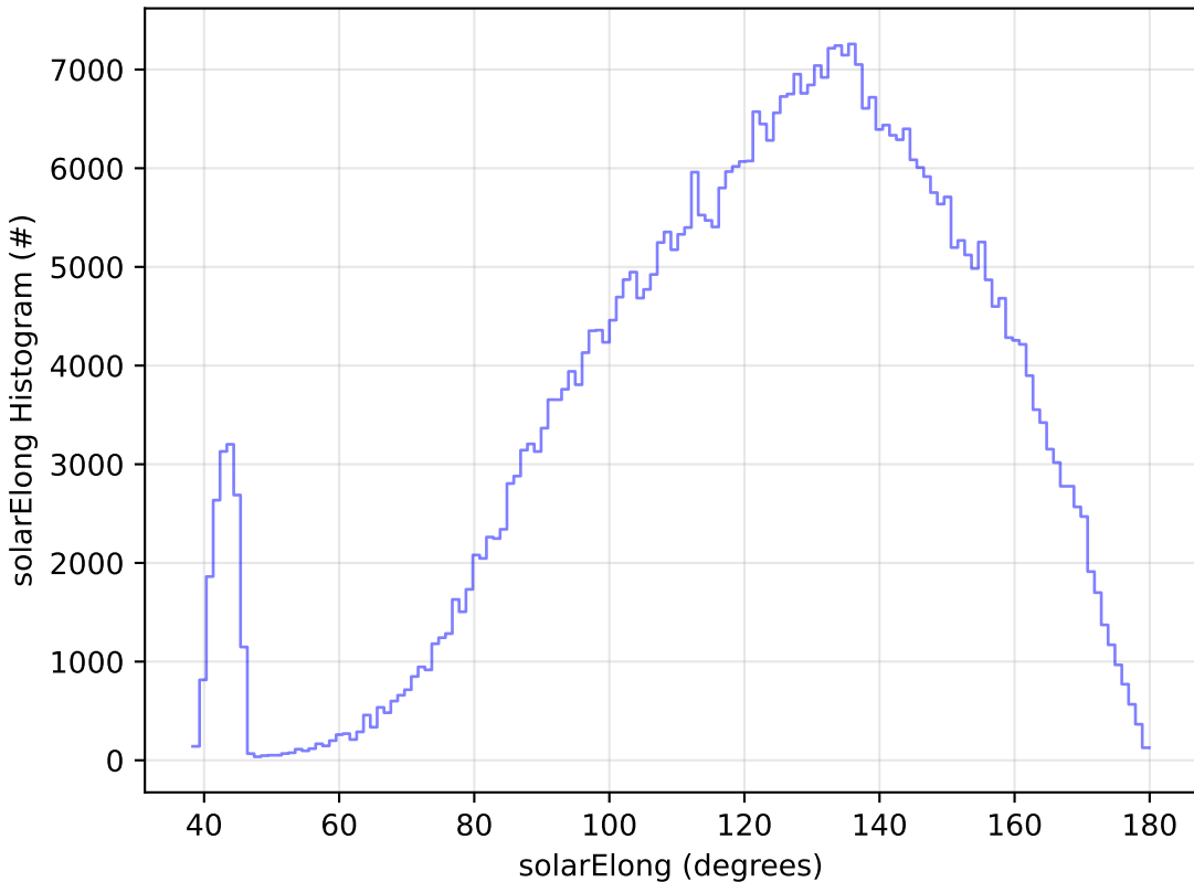
ddf_acor_sf15_lsf20_lsr20_v3.4_10yrs All sky r band: solarElong Histogram
