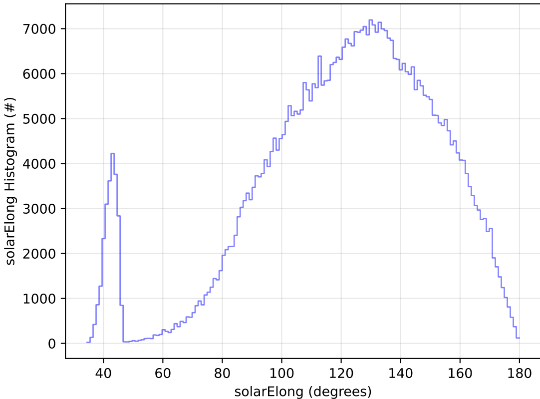
ddf_acor_sf15_lsf20_lsr20_v3.4_10yrs All sky i band: solarElong Histogram
