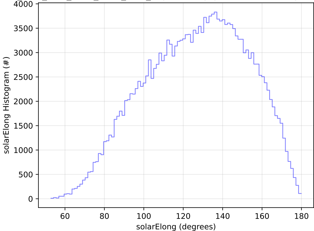
ddf_acor_sf15_lsf20_lsr20_v3.4_10yrs All sky g band: solarElong Histogram
