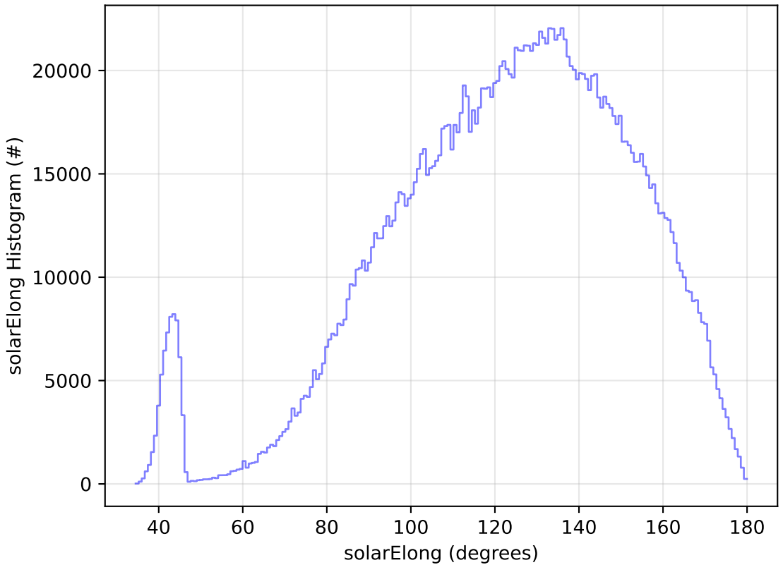
ddf_acor_sf15_lsf20_lsr20_v3.4_10yrs All sky all bands: solarElong Histogram
