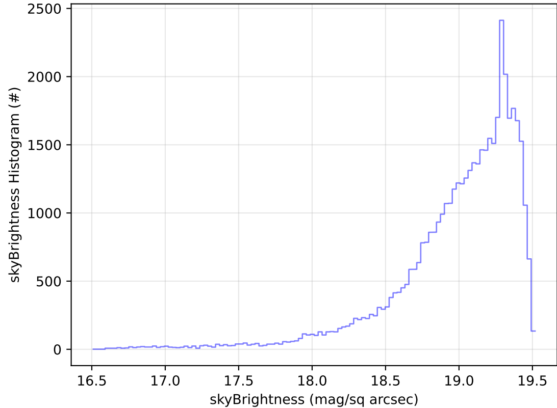
ddf_acor_sf15_lsf20_lsr20_v3.4_10yrs Yr 1 z band: skyBrightness Histogram
