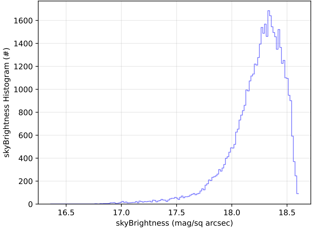
ddf_acor_sf15_lsf20_lsr20_v3.4_10yrs Yr 1 y band: skyBrightness Histogram
