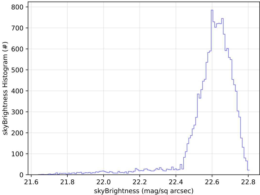
ddf_acor_sf15_lsf20_lsr20_v3.4_10yrs Yr 1 u band: skyBrightness Histogram
