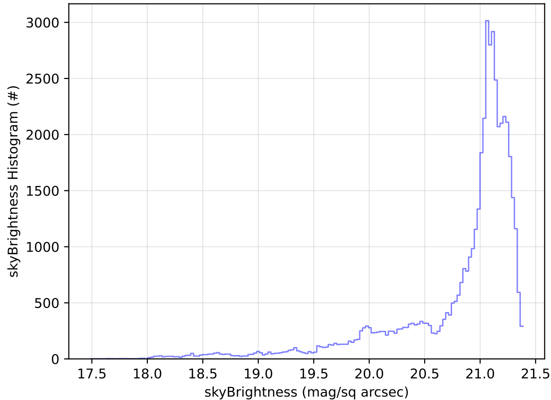
ddf_acor_sf15_lsf20_lsr20_v3.4_10yrs Yr 1 r band: skyBrightness Histogram
