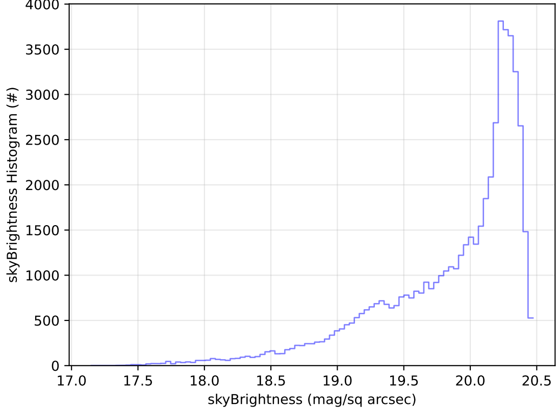
ddf_acor_sf15_lsf20_lsr20_v3.4_10yrs Yr 1 i band: skyBrightness Histogram
