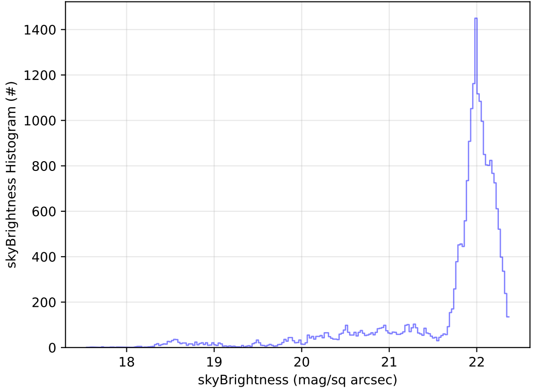
ddf_acor_sf15_lsf20_lsr20_v3.4_10yrs Yr 1 g band: skyBrightness Histogram
