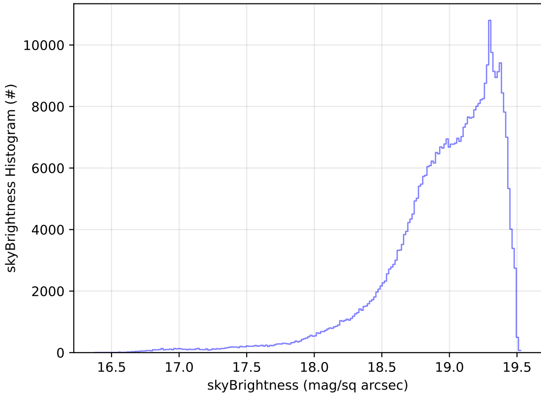
ddf_acor_sf15_lsf20_lsr20_v3.4_10yrs WFD z band: skyBrightness Histogram
