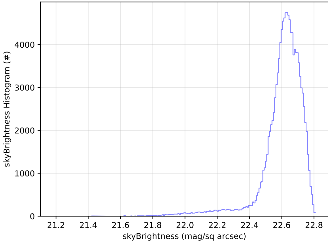
ddf_acor_sf15_lsf20_lsr20_v3.4_10yrs WFD u band: skyBrightness Histogram
