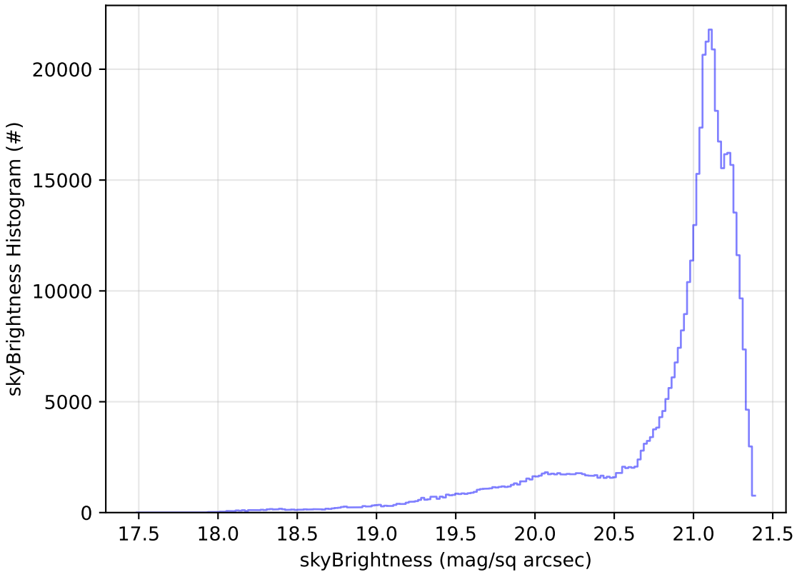
ddf_acor_sf15_lsf20_lsr20_v3.4_10yrs WFD r band: skyBrightness Histogram
