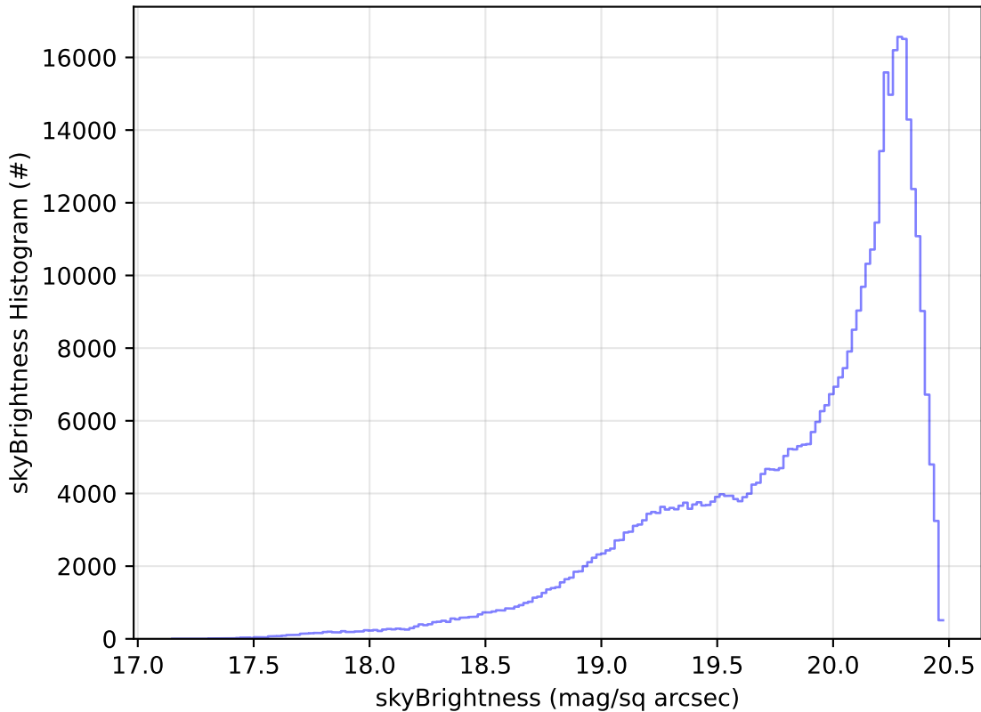
ddf_acor_sf15_lsf20_lsr20_v3.4_10yrs WFD i band: skyBrightness Histogram
