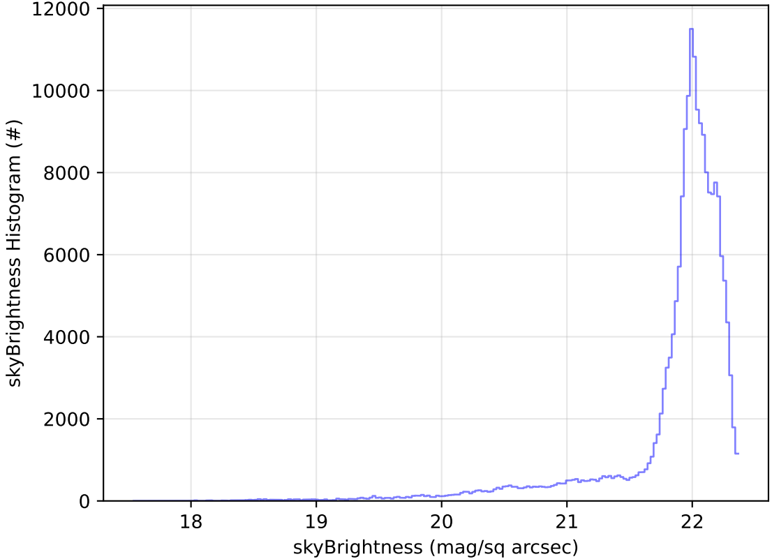
ddf_acor_sf15_lsf20_lsr20_v3.4_10yrs WFD g band: skyBrightness Histogram
