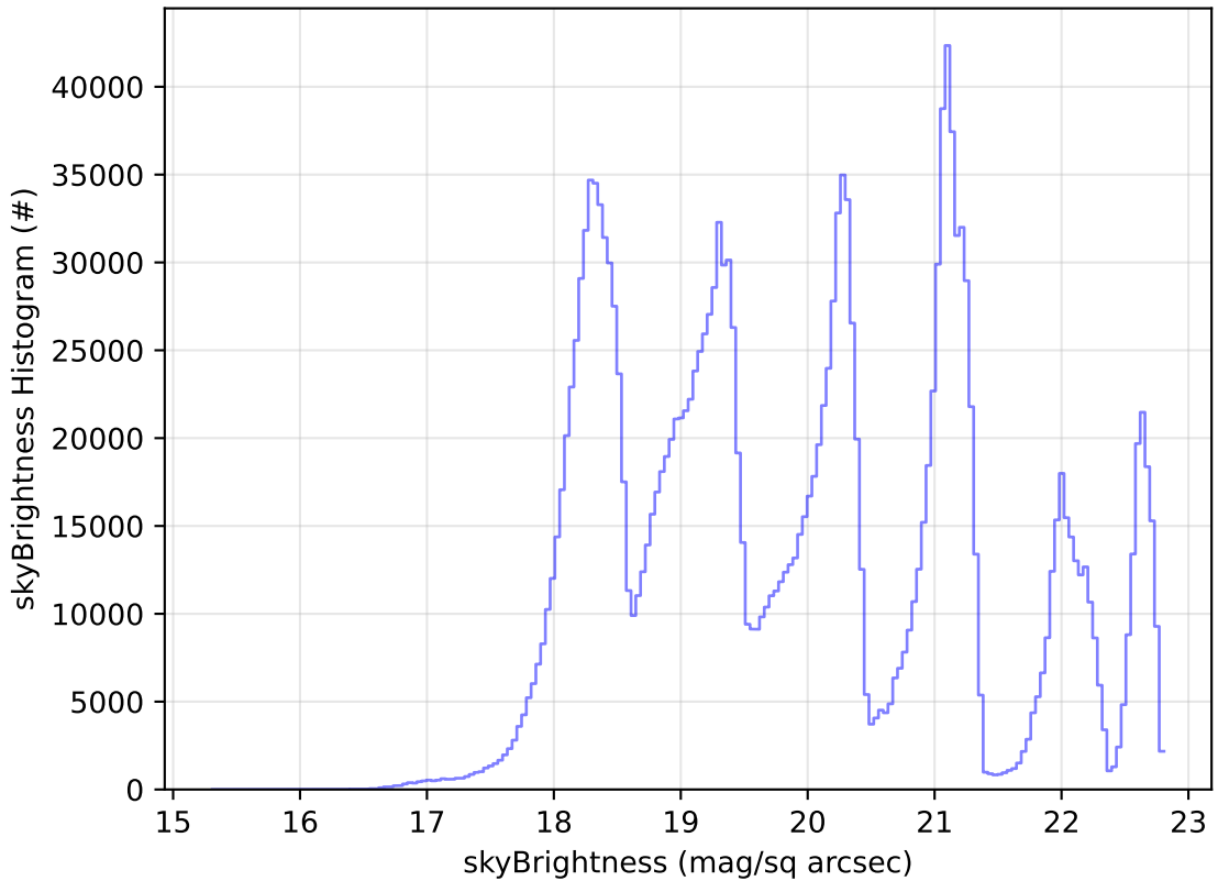
ddf_acor_sf15_lsf20_lsr20_v3.4_10yrs WFD all bands: skyBrightness Histogram
