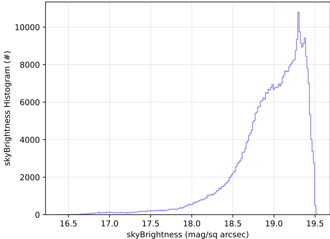
ddf_acor_sf15_lsf20_lsr20_v3.4_10yrs All sky z band: skyBrightness Histogram
