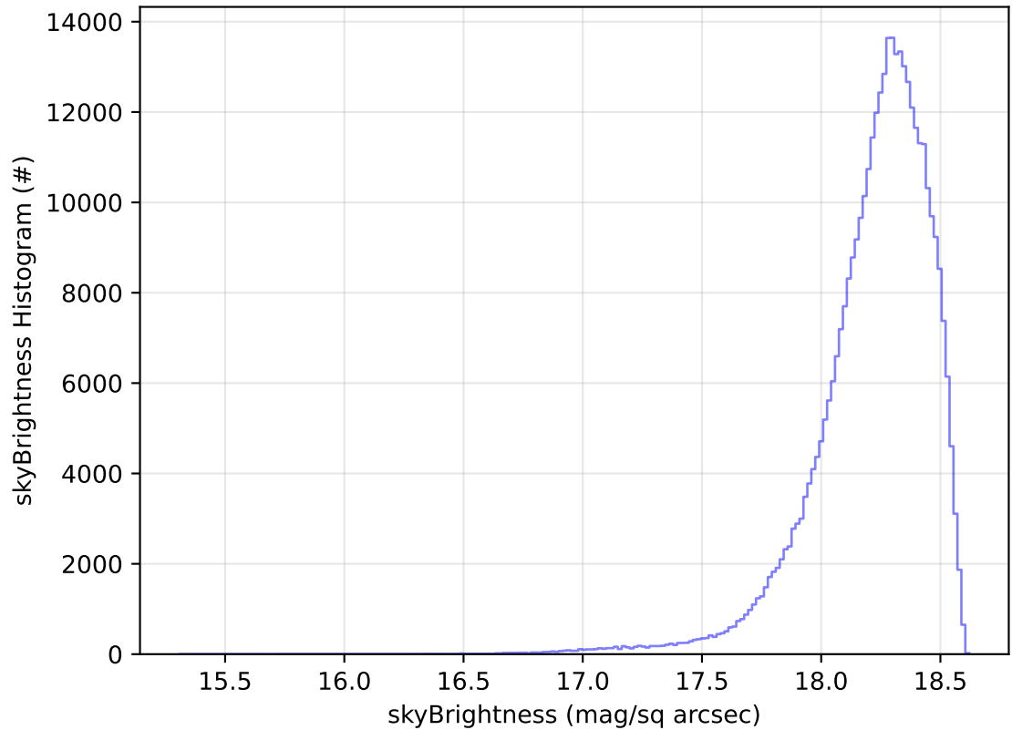
ddf_acor_sf15_lsf20_lsr20_v3.4_10yrs All sky y band: skyBrightness Histogram
