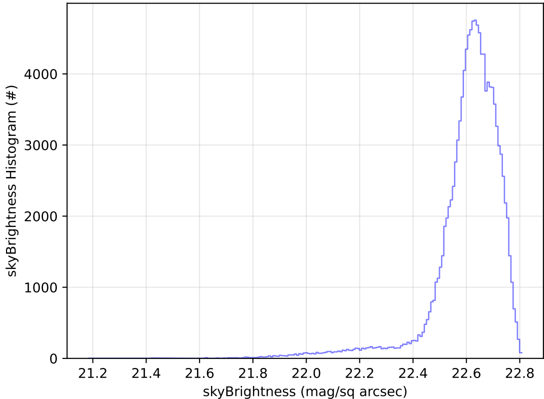
ddf_acor_sf15_lsf20_lsr20_v3.4_10yrs All sky u band: skyBrightness Histogram
