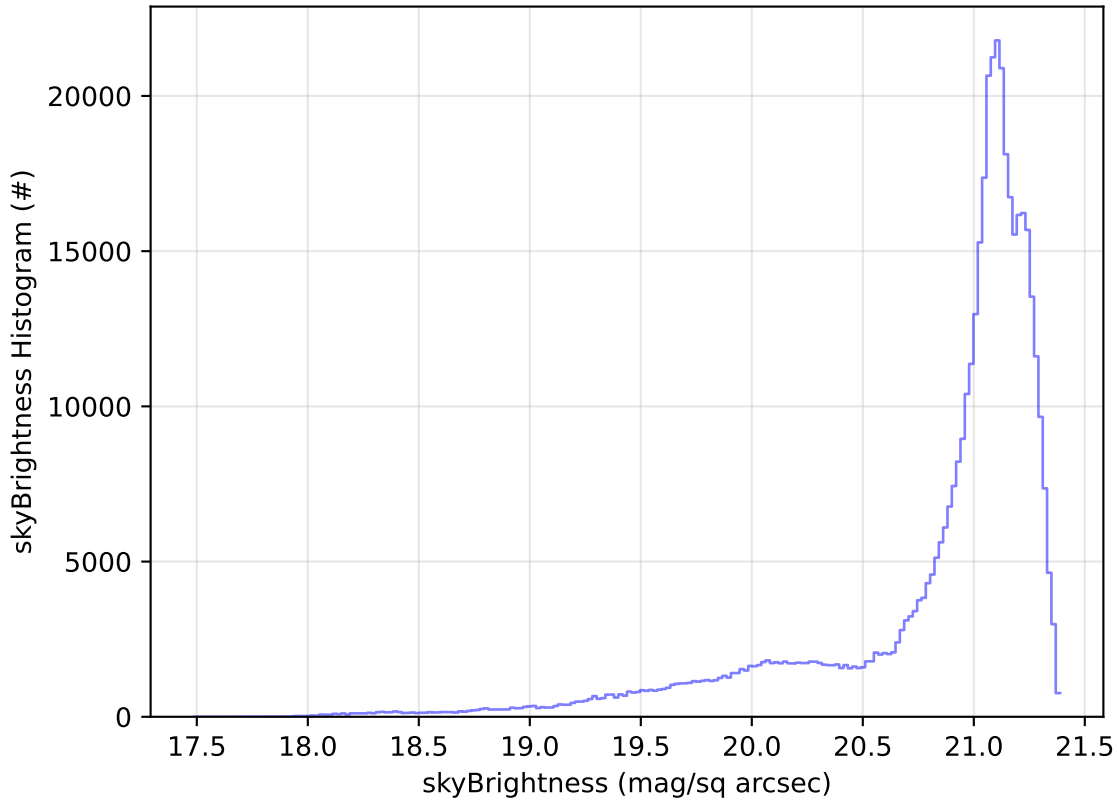
ddf_acor_sf15_lsf20_lsr20_v3.4_10yrs All sky r band: skyBrightness Histogram
