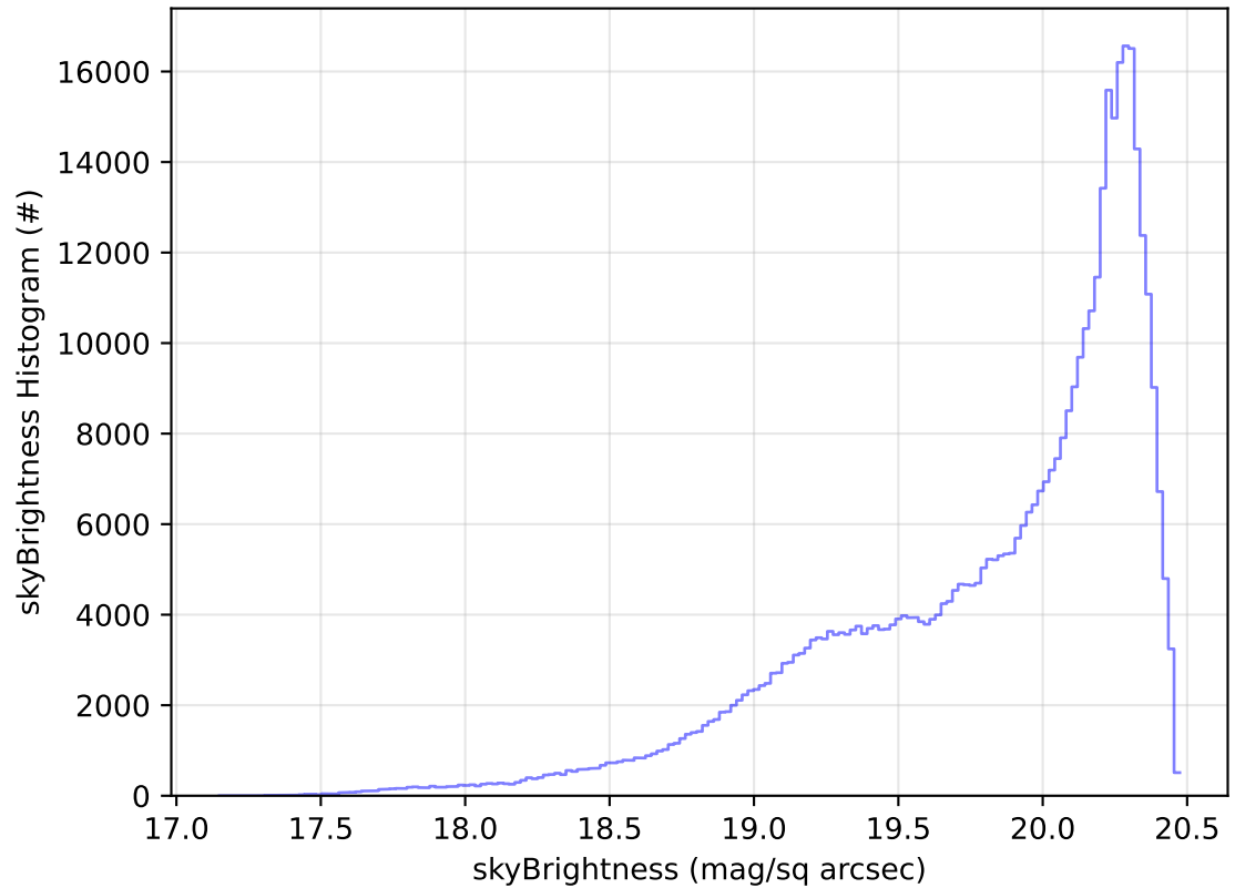
ddf_acor_sf15_lsf20_lsr20_v3.4_10yrs All sky i band: skyBrightness Histogram
