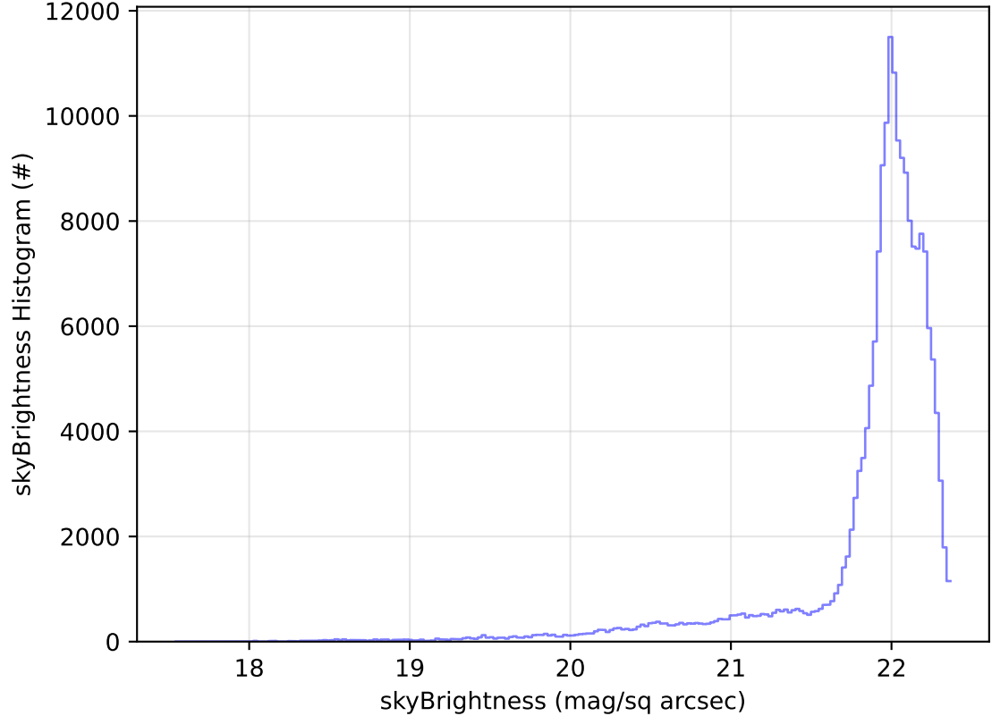
ddf_acor_sf15_lsf20_lsr20_v3.4_10yrs All sky g band: skyBrightness Histogram
