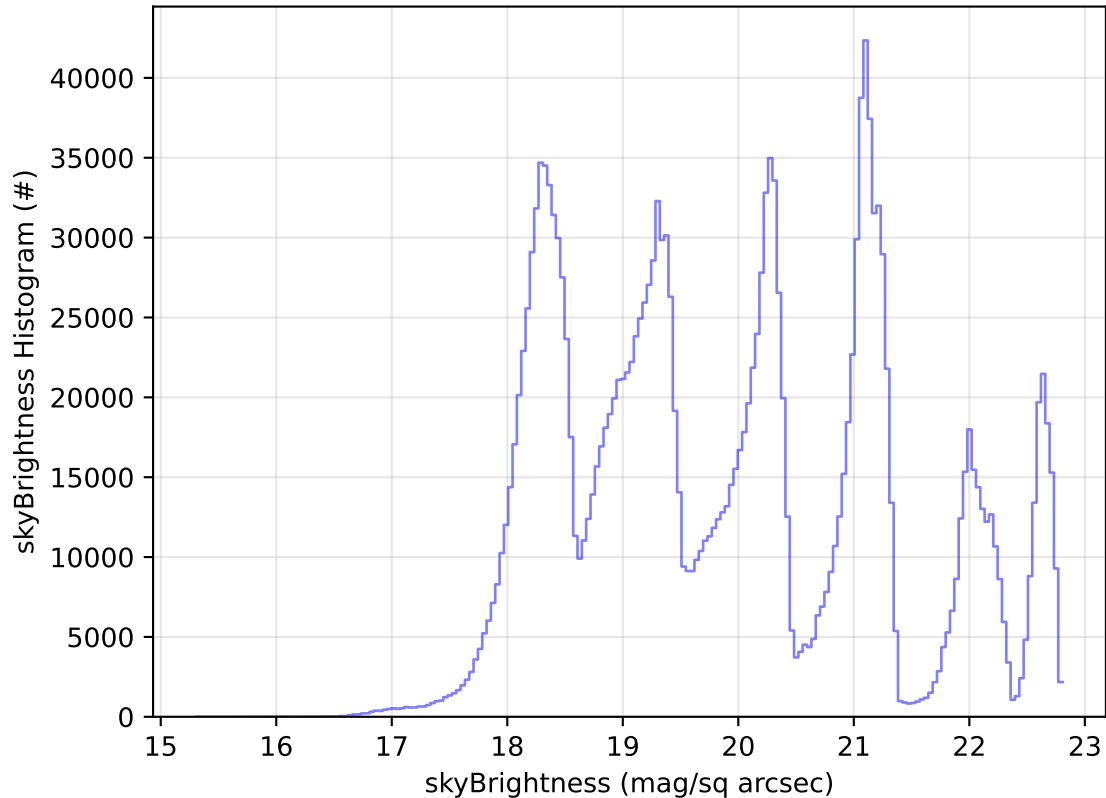
ddf_acor_sf15_lsf20_lsr20_v3.4_10yrs All sky all bands: skyBrightness Histogram
