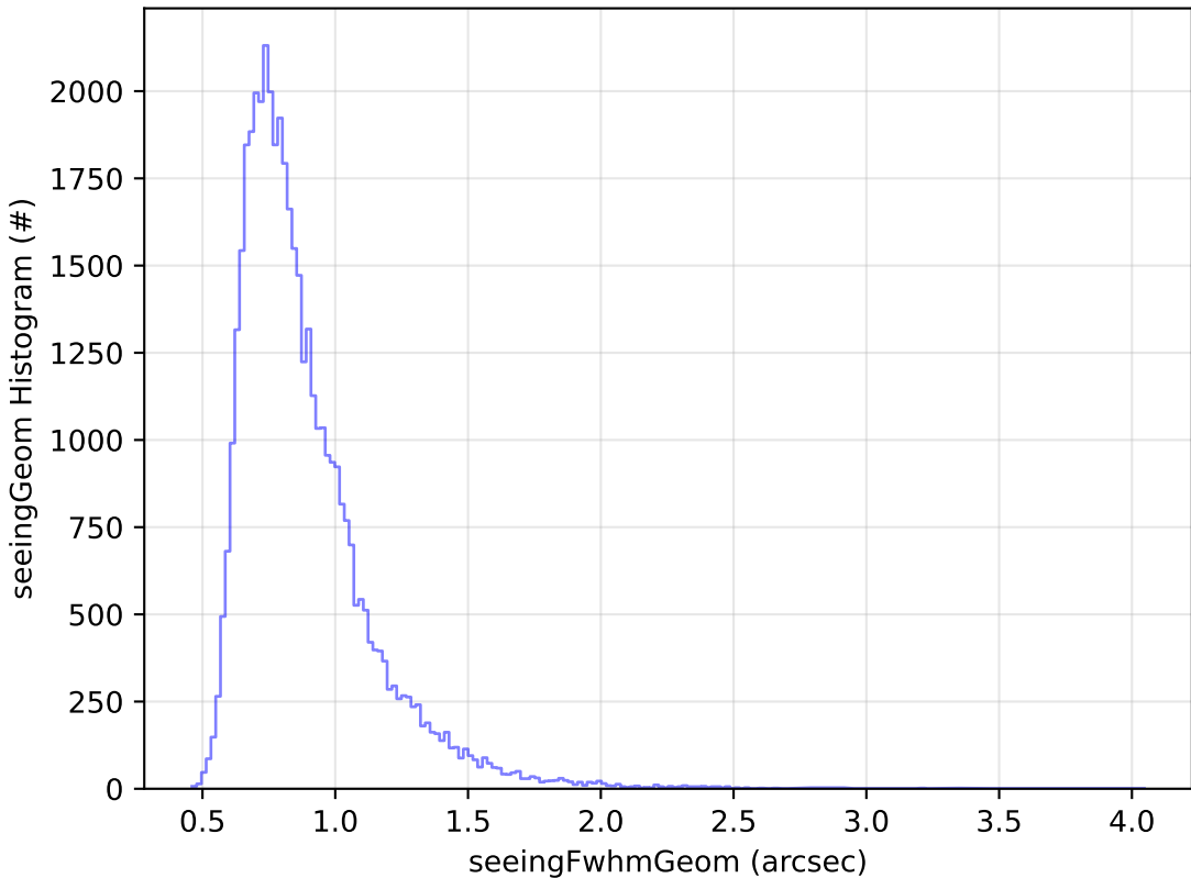
ddf_acor_sf15_lsf20_lsr20_v3.4_10yrs Yr 1 z band: seeingGeom Histogram
