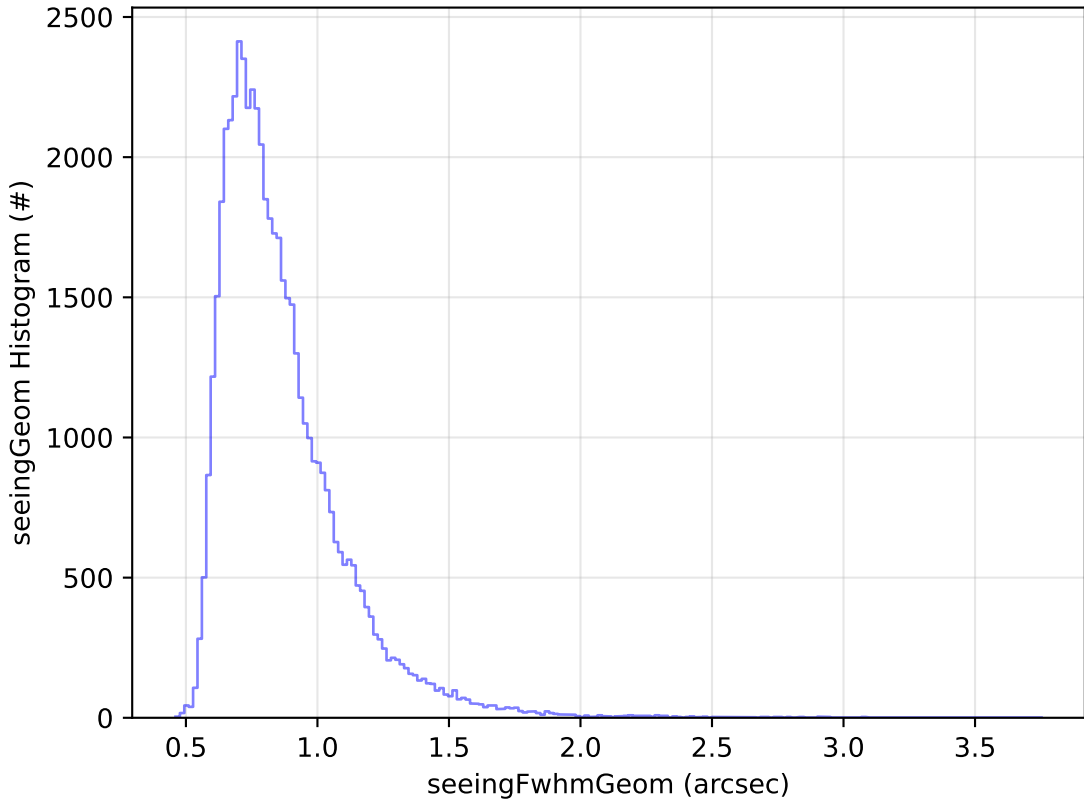
ddf_acor_sf15_lsf20_lsr20_v3.4_10yrs Yr 1 i band: seeingGeom Histogram
