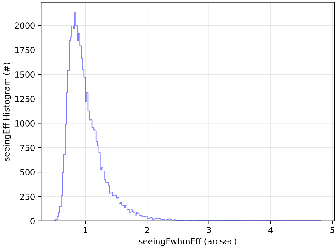
ddf_acor_sf15_lsf20_lsr20_v3.4_10yrs Yr 1 z band: seeingEff Histogram
