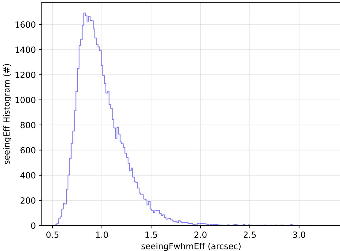
ddf_acor_sf15_lsf20_lsr20_v3.4_10yrs Yr 1 y band: seeingEff Histogram
