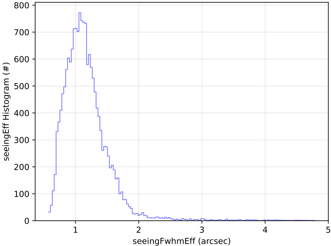
ddf_acor_sf15_lsf20_lsr20_v3.4_10yrs Yr 1 u band: seeingEff Histogram
