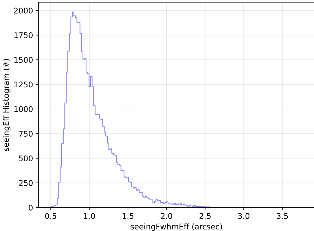
ddf_acor_sf15_lsf20_lsr20_v3.4_10yrs Yr 1 r band: seeingEff Histogram
