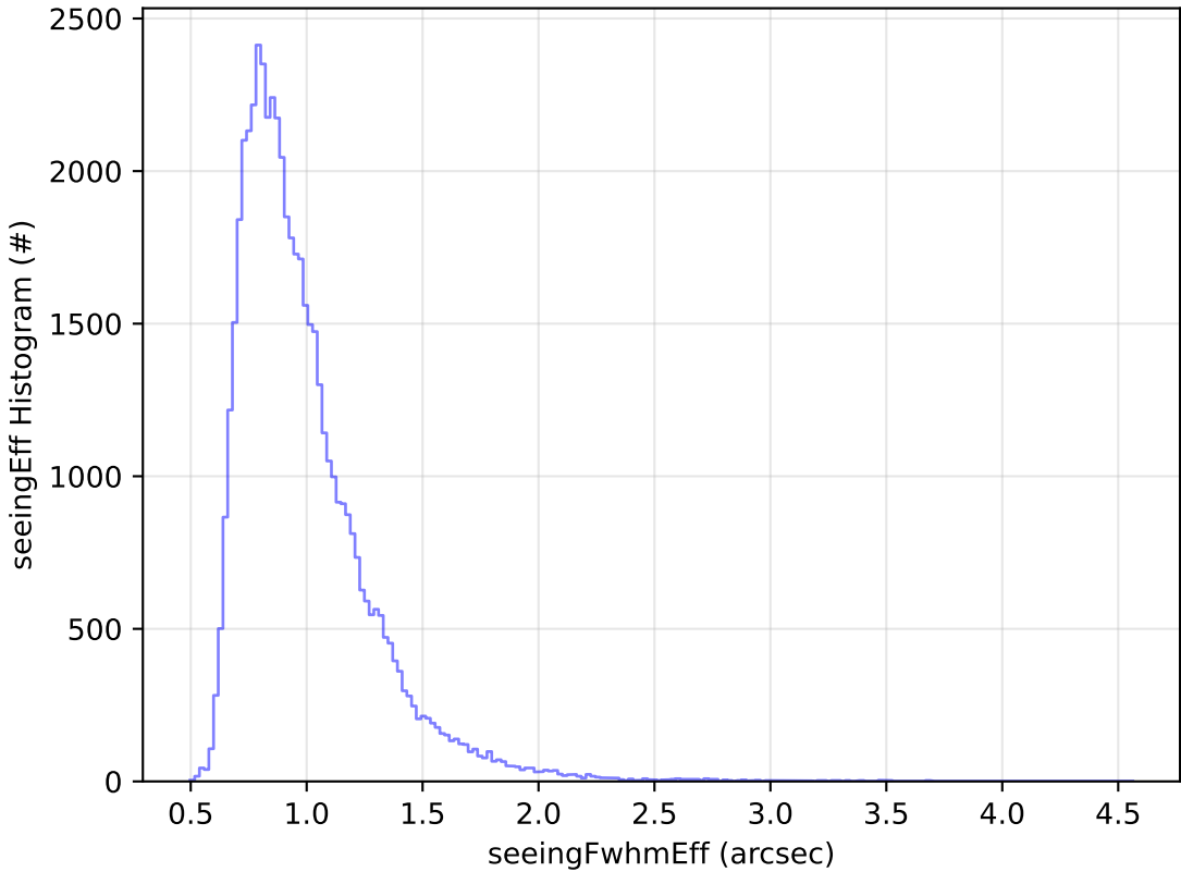
ddf_acor_sf15_lsf20_lsr20_v3.4_10yrs Yr 1 i band: seeingEff Histogram
