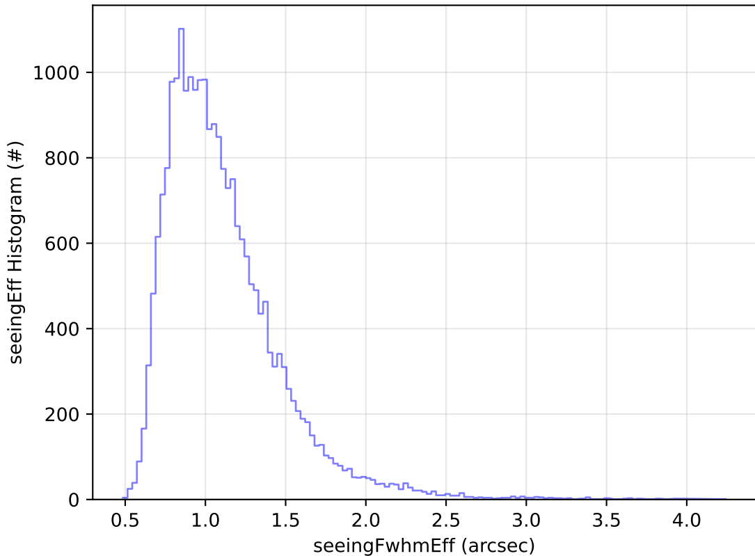
ddf_acor_sf15_lsf20_lsr20_v3.4_10yrs Yr 1 g band: seeingEff Histogram
