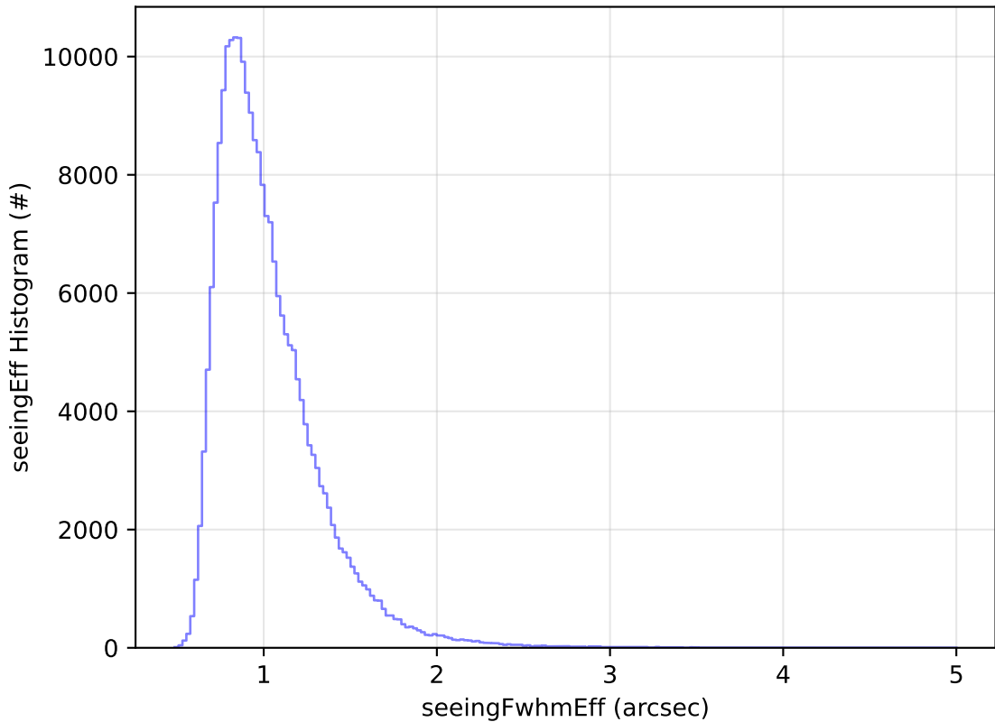
ddf_acor_sf15_Isf20_Isr20_v3.4_10yrs Yr 1 all bands: seeingEff Histogram
