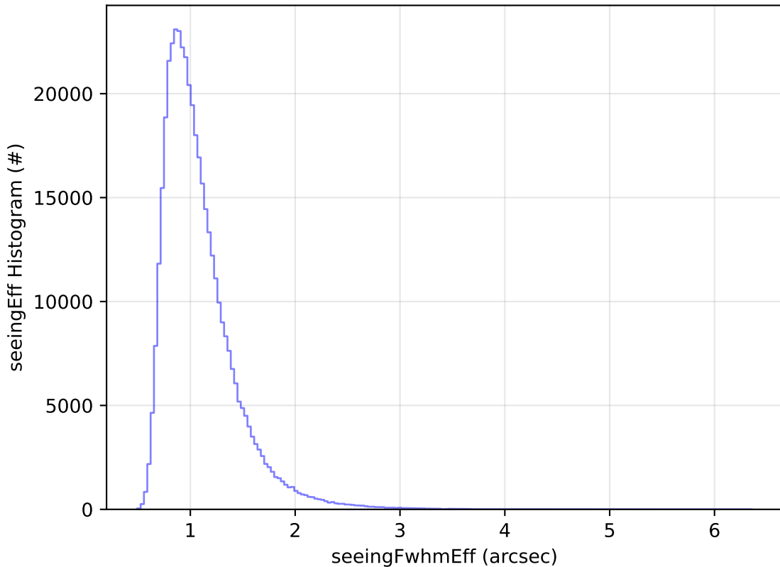
ddf_acor_sf15_lsf20_lsr20_v3.4_10yrs WFD z band: seeingEff Histogram
