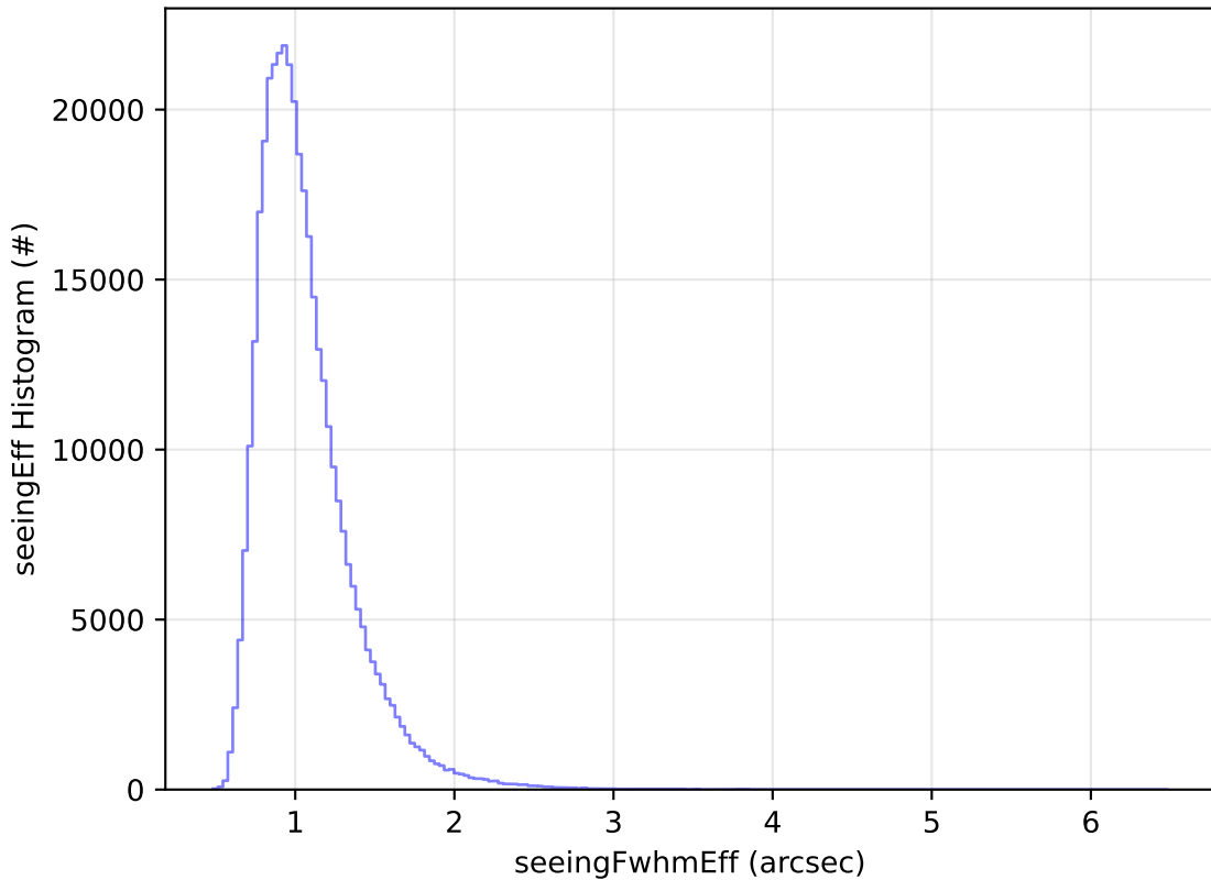
ddf_acor_sf15_lsf20_lsr20_v3.4_10yrs WFD y band: seeingEff Histogram
